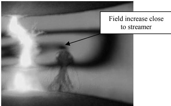
Fig. 3. Kerrogram and inherent glow of discharge. Voltage U= 132 kV, gap d= 3.5 mm. The moments of Kerr picture and breakdown were the same t_k \approx t_b = 1.4 \mu sec. Electric field strength at the centre of the gap E \approx 720 kV/cm.
