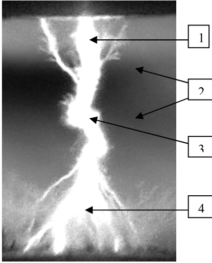
Fig. 2. Discharge channel in case of screened electrodes. Kerrogram and inherent glow of discharge. Voltage U= 145 kV, gap d= 4 mm. Kerr picture was obtained at t_k = 1.45 \mu sec, breakdown occurred at t_b = 1.7 \mu sec. 1 – anode streamer, 2 - Kerr darkening, 3- the place of breakdown origin, 4 - cathode streamer
