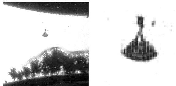
Fig. 1. Shadow photo (a): top, modified anode; bottom, metallic cathode; U = 142 \text{ kV} , d = 3 \text{ mm} , t = 2.05 \mu\text{s} ; dark points are microparticles; (b) enlarged part of the interelectrode gap with the nonelectrode streamer.
